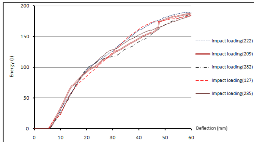
Fig. 6. Energy-Deflection curves from the impact bending models of the composite hat-shapes
